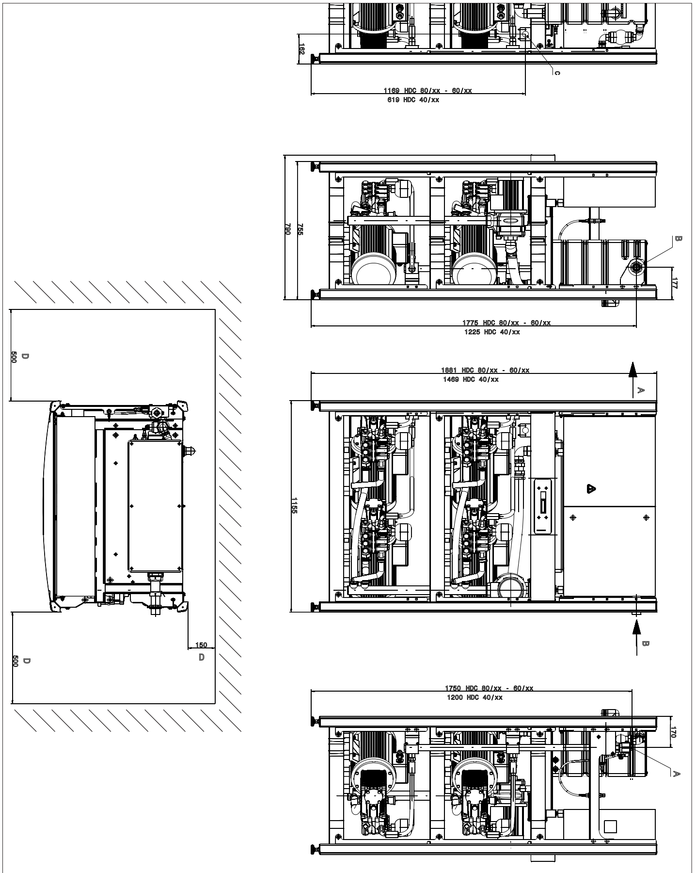
Figur HDC 80/16 H uten kleddingsplater
